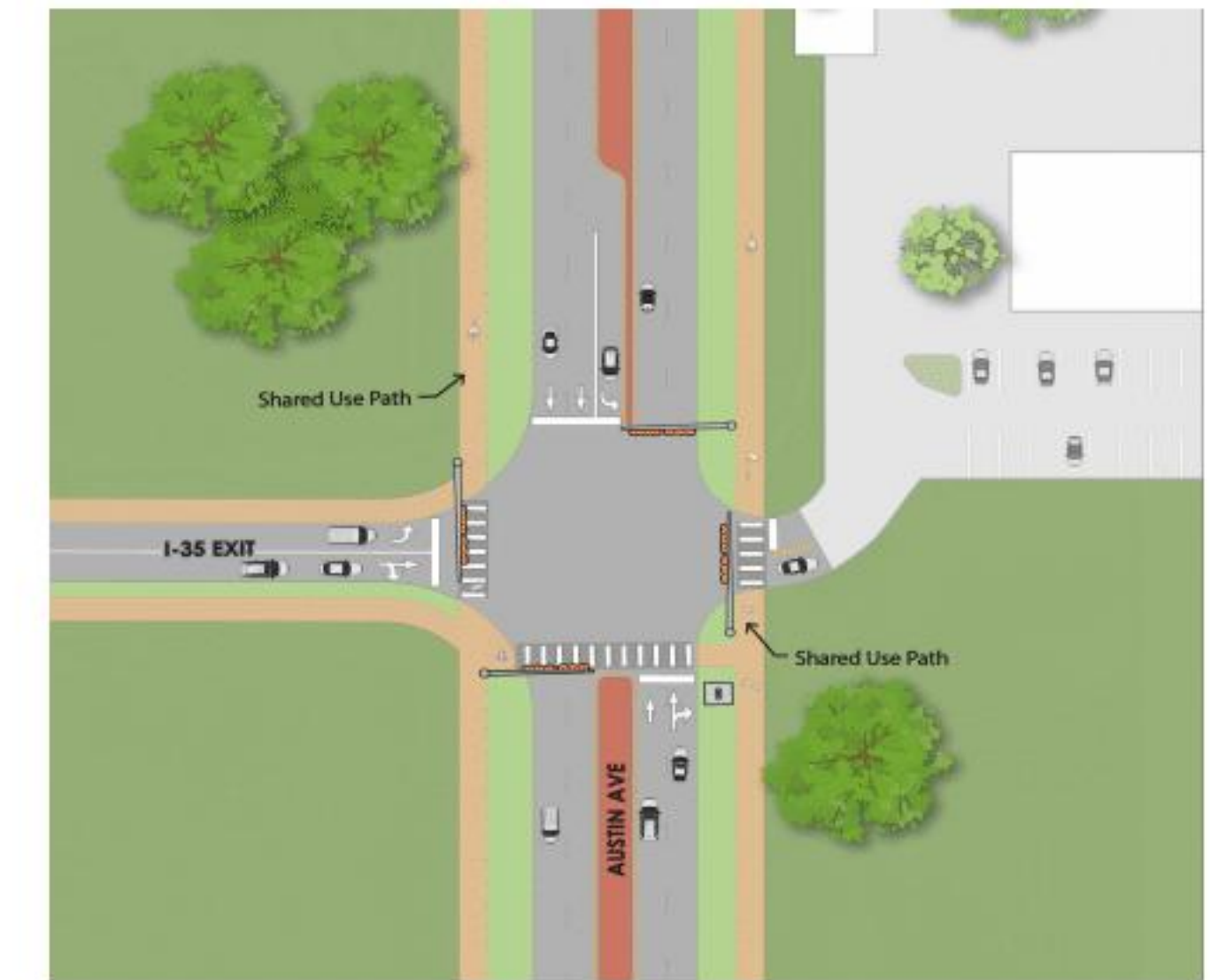
Austin Ave. at I-35 Concept
