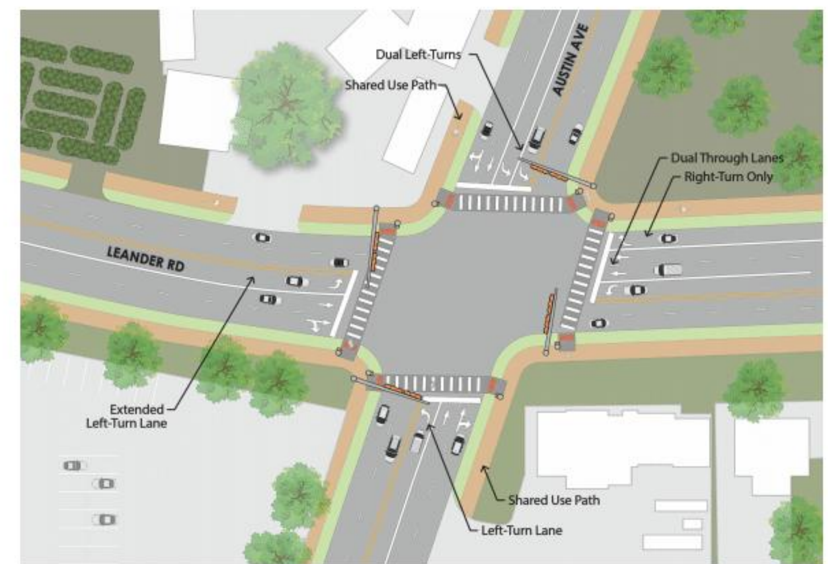
Austin Ave. at Leander Road Concept
